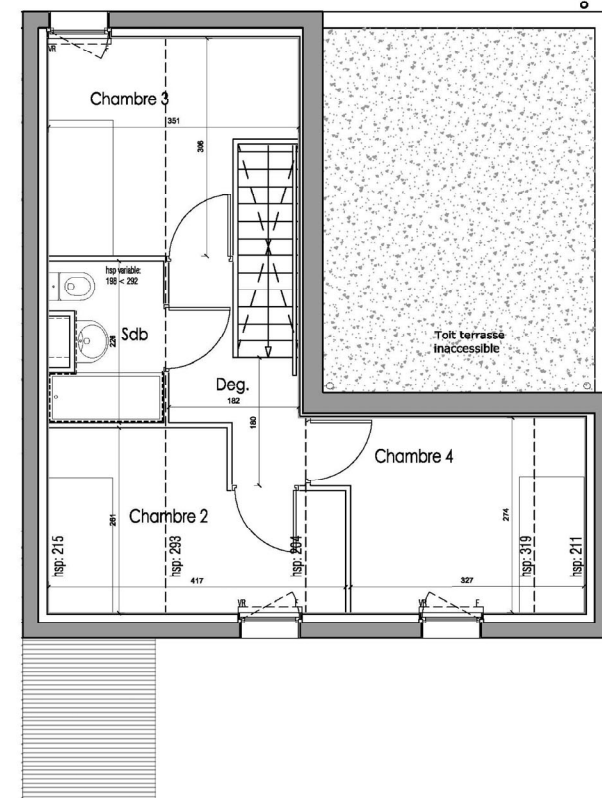
Plan R+1
